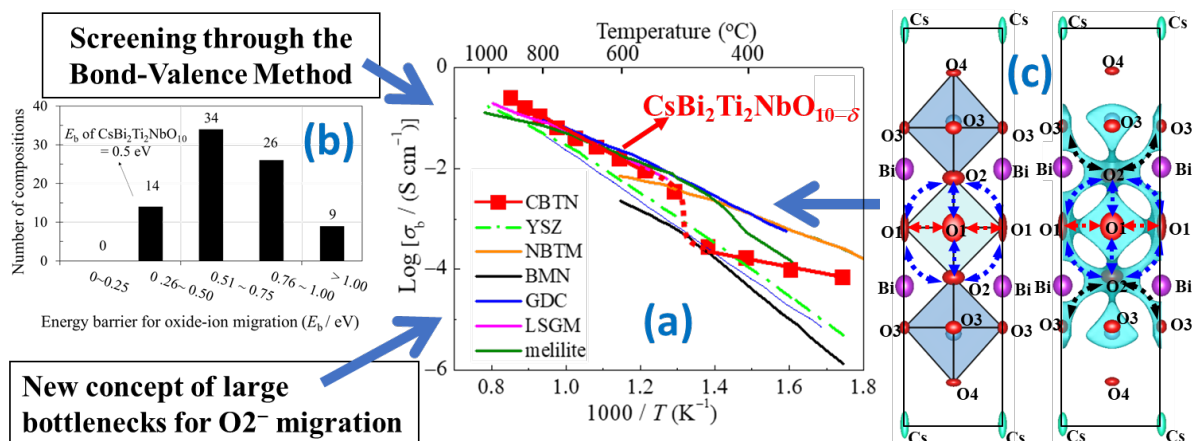
Figure 1. The mechanism, design concept, and structural characteristics that afford high oxide-ion conductivity in \text{CsBi}_2\text{Ti}_2\text{NbO}_{10-\delta}
