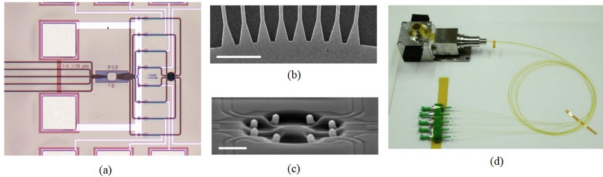
Figure 1. Orbital angular momentum Multiplexer/Demultiplexer
