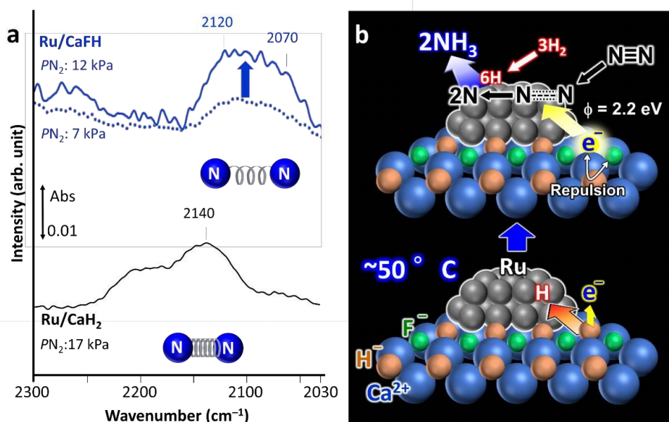
Figure 2. Spectroscopic measurement results and possible reaction mechanism a) Fourier Transform Infrared (FT-IR) spectra for nitrogen adsorption on the developed fluoride-containing Ru/CaFH catalyst (top) showing weakened bond between nitrogen atoms compared with a non-modified Ru/CaH 2 catalyst (lower spectrum). b) Proposed reaction mechanism using the Ru/CaFH catalyst.
