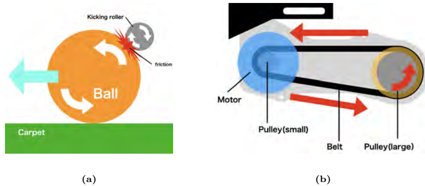
Fig. 3: Structure of Kicker
