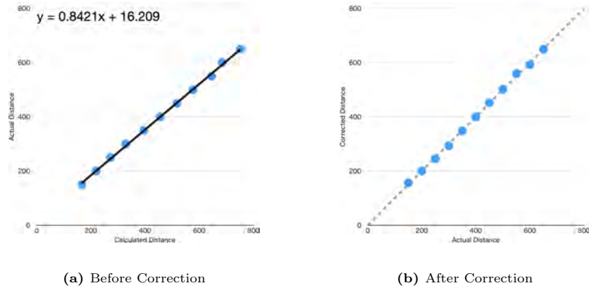
Fig. 5: Relationship between Actual Distance and Calculated Distance
